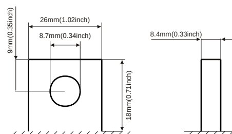
Terminal Dimensions
